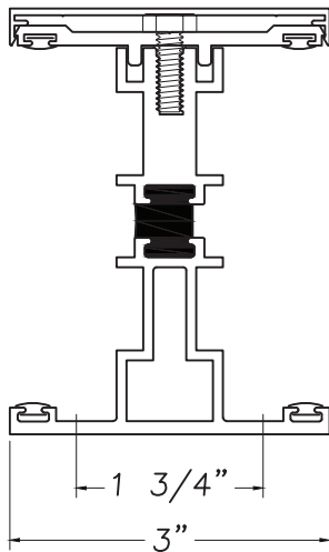
RSM Mullion M21045 (Mull) M21043 (Base) M21044 (Cap)
