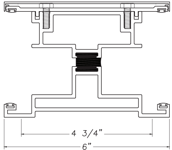
6" T-MULLION & COVER PT# M21344 (T-MULL) PT# M21343 (BASE) PT# M22342 (CAP)
