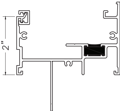
Subsill W/Fin M21012 (Sill) CE-13986 (C-Mull)
