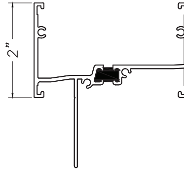
Subsill W/Fin M17032
