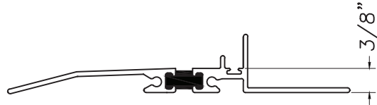
Flashing / Subsill M541227
