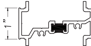
Subsill or Stack Mull M25615
