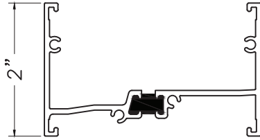
Subsill & Spacer M16318
