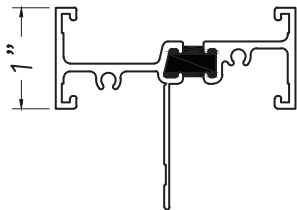
Spacer Mull or Stack Mull M43325
